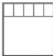
STORE WINDOW 98" W x 102" H 1.13" x 1.155" OPENING
