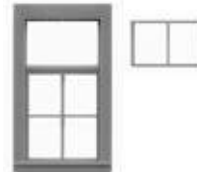
6 PANE WINDOW WITH 2 PANE TILT OUT SASH 34" W x 64" H .44" x .78" OPENING
