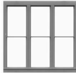
TRIPLE UNIT 8096 100" W x 92" H 1.18" x 1.1" OPENING
