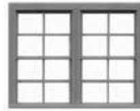
4/4 DBL DBL HUNG WINDOW 80" W x 62" H .955" x .76" OPENING
