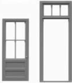
4 LITE DOOR/TRANSOM 39" W x 92" H .5" x 1.35" OPENING TTG #8119 3 SETS $3.50
