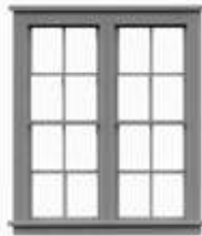
DOUBLE OF 8030 64" W x 80" H .81" x .98" OPENING
