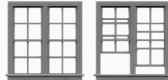
DOUBLE UNIT OF 8028/8069 60" W x 62" H .75" x .78" OPENING
