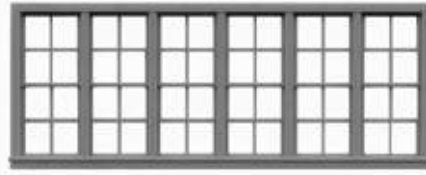
SIX UNIT 4/4 DBL HUNG WINDOW TRIPLE OF 8064 180" W x 64" H 2.11" x .80" OPENING
