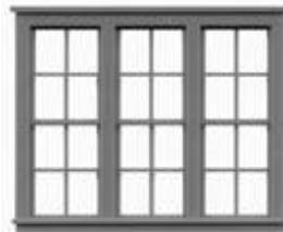
TRIPLE OF 8030 98" W x 80" H 1.225" x .98" OPENING
