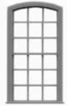
9/9 DBL HUNG ARCH TOP WINDOW 44" W x 90" H .54" x 1.07" OPENING
