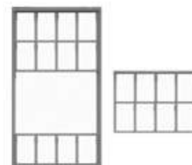
25 PANE TILT OUT WINDOW 60" W x 104" H .68" x 1.19" OPENING
